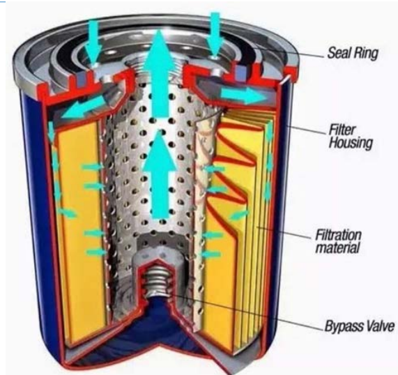
ANATOMY & WORKING OF AN OIL FILTER
